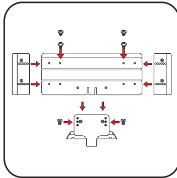
Slide Bracket
