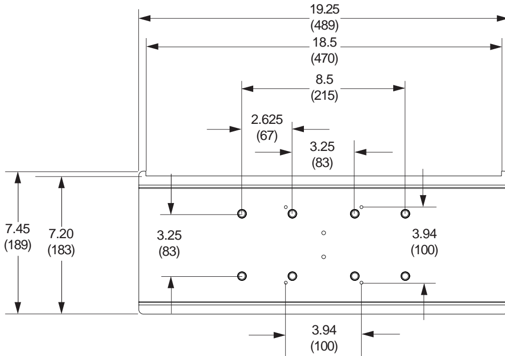
SIDE VIEW
