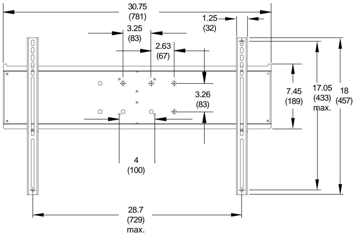
ADAPTER BRACKET DETAIL
