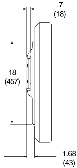
SIDE VIEW WITH DEEP BRACKET
