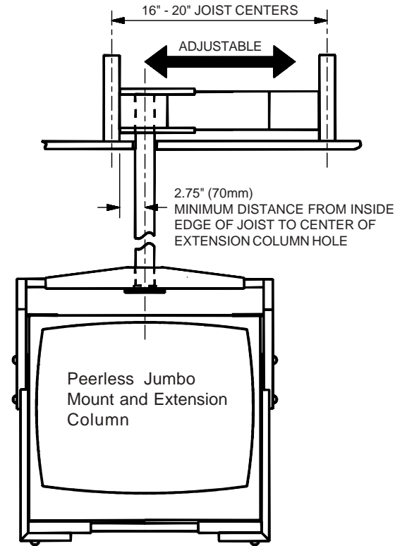
FRONT VIEW Peerless Jumbo Mount attached to Internal Joist Mount.
