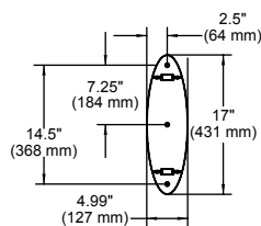
WALL PLATE DETAIL
