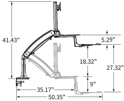
Base reach & range (side)
