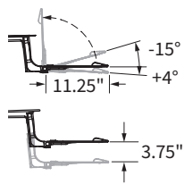
Keyboard platform tilt & range
