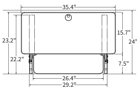
Height & width
