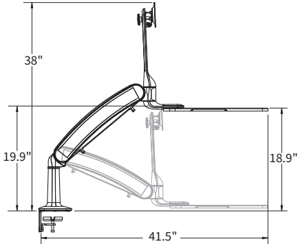
Base reach & range (side)
