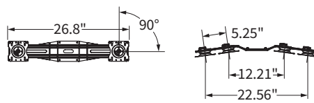
Dual Monitor Adaptor option
