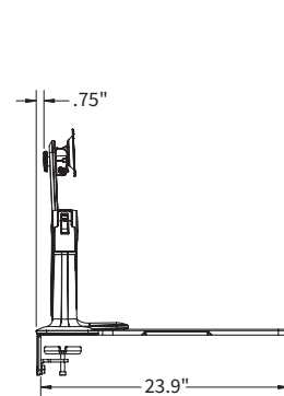
Stowed depth
