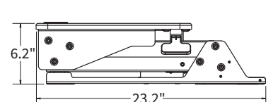
Stowed Depth
