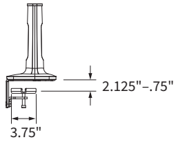
Base C-Clamp
