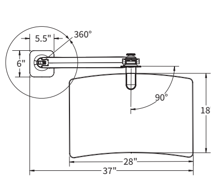
Pivot (top)
