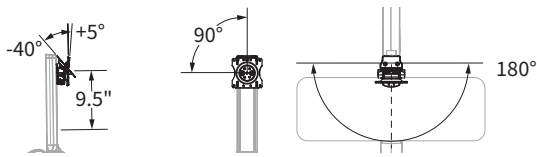
Monitor Mount tilt, rotate & swivel
