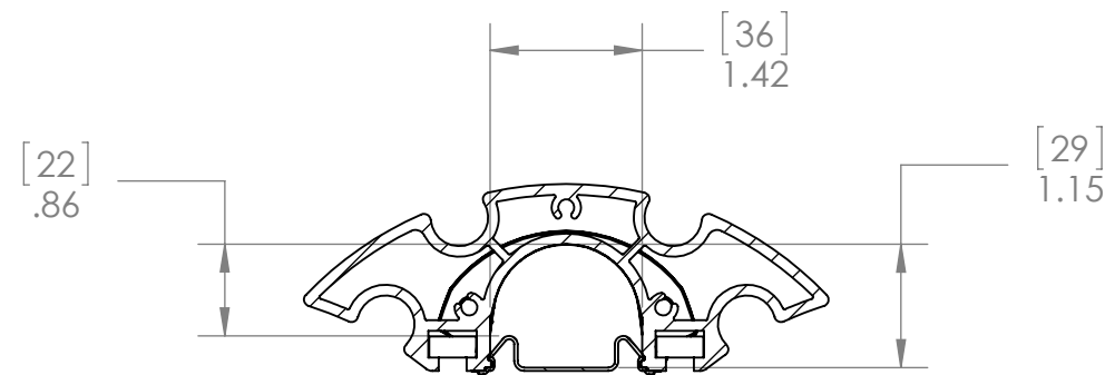
SECTION A-A SCALE 1 : 2 CABLE CHANNEL DIMENSIONS THRU ARM
