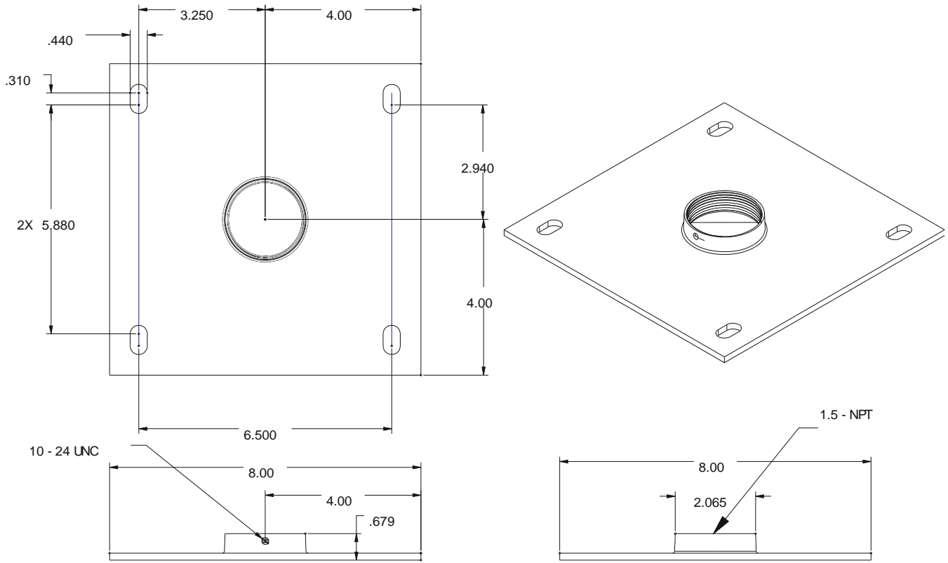
Figure 2. CMA-110 Dimensions
