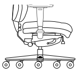
HL Low Desk Height 15¼" - 18" -2¼" for ST mechanism, no SD.
