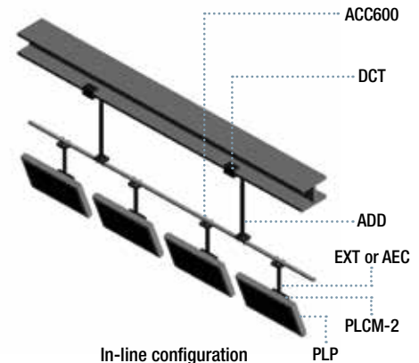
In-line configuration
