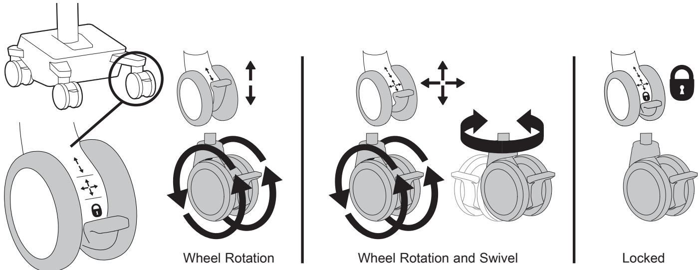
3 Function Caster
