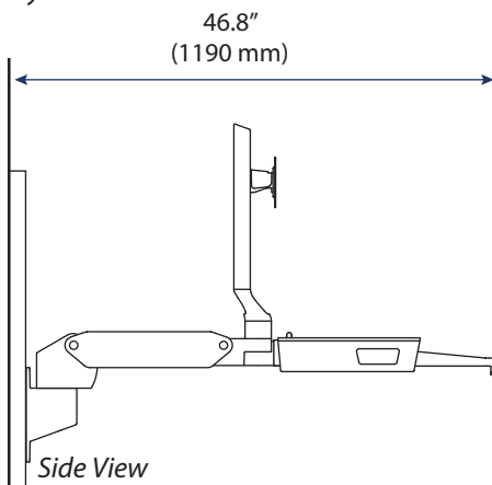
Fully Extended
