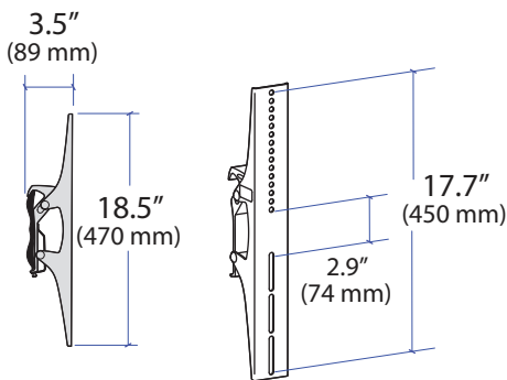
Display Mount Vertical Hole Spacing 100 mm to 450 mm
