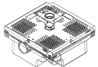
360° (±180°) YAW
