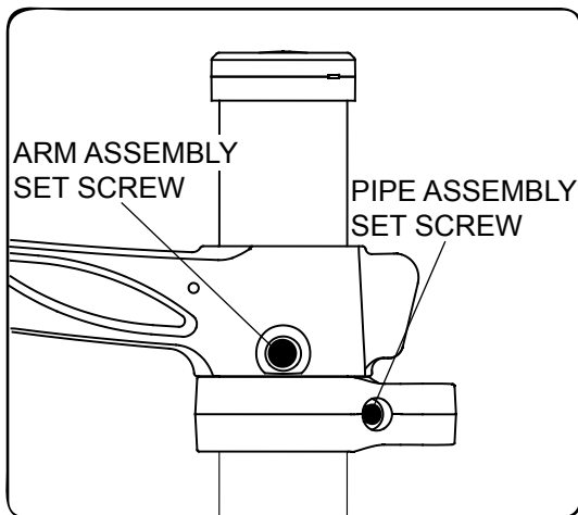
DETAIL 2
